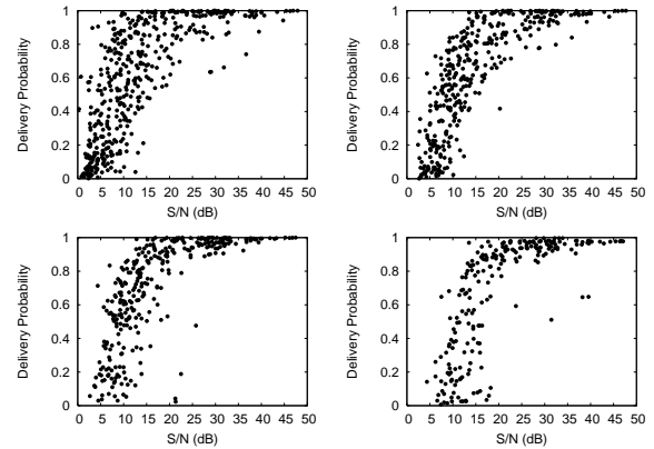
Figure 14: Delivery probability at 1, 2, 5.5, and 11 Mbit/s versus the average S/N. Each data point represents an individual transmitter-receiver pair.
