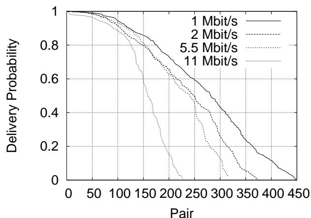
Figure 4: The distribution of link delivery probabilities for 1500-byte packets. Each point corresponds to one sender/receiver pair at a particular bit-rate. Points were restricted to pairs that managed to exchange at least one packet during the experiment. Most pairs have intermediate delivery probabilities.
