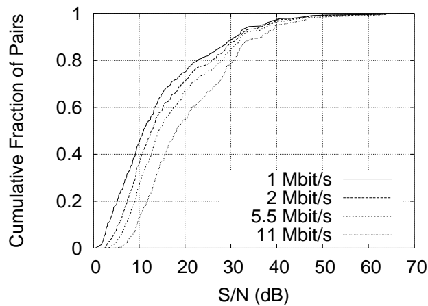
Figure 13: Distribution of Roofnet links' average S/N values, for the same experiments as Figure 4. There is one value in the CDF per send/receive pair.
