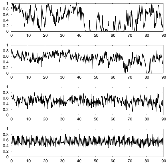
Figure 7: Delivery probability over time (in seconds) for four 1 Mbit/s links, all with about 50% average loss rate. The send rate is about 80 1500-byte packets/second. Each point is an average over 200 milliseconds. The top graph shows one of Roofnet's most bursty links, the bottom one of the least bursty.
